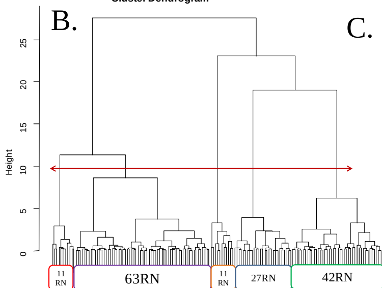
Cluster Dendrogram
